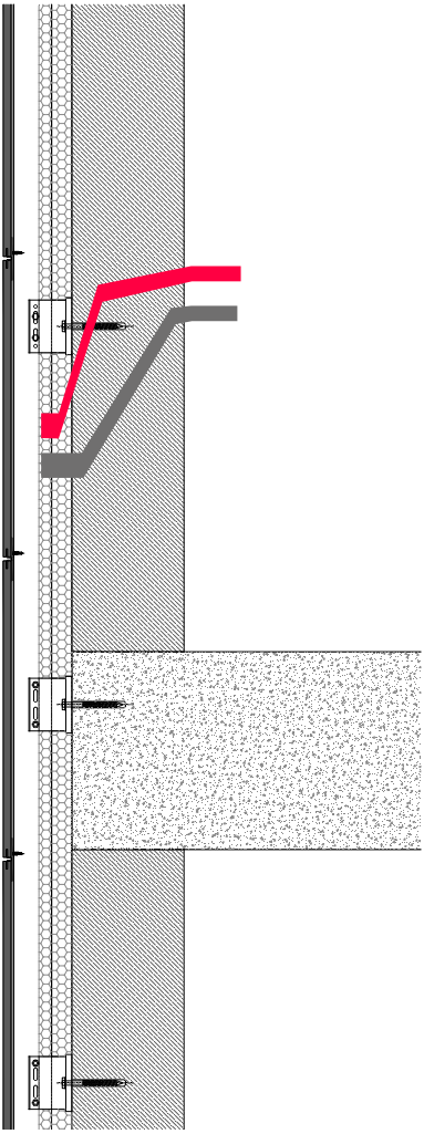
FACHADA VENTILADA VENTILATED FACADE
